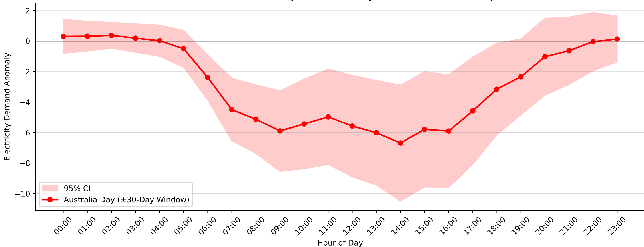
Castle Cove Demand Anomaly: Australia Day (2004–2017, \pm 30 -Day Window)
